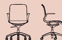
EX5 L 67 x W 72 x H 90 cm
