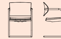
406B L 54 x W 49 x H 81 cm
