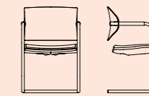
406B Mesh L 54 x W 49 x H 81 cm
