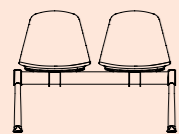
EP14 L 105 x W 60 x H 78 cm
